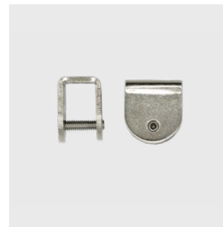
Anchor D to hang 9-12 mm thickness direct ceiling panel with steel cable. — 20 x 20 x 15 mm
